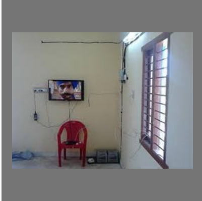
Solar DC Ceiling Fan DC Tubelight Appliances- Inverterless
